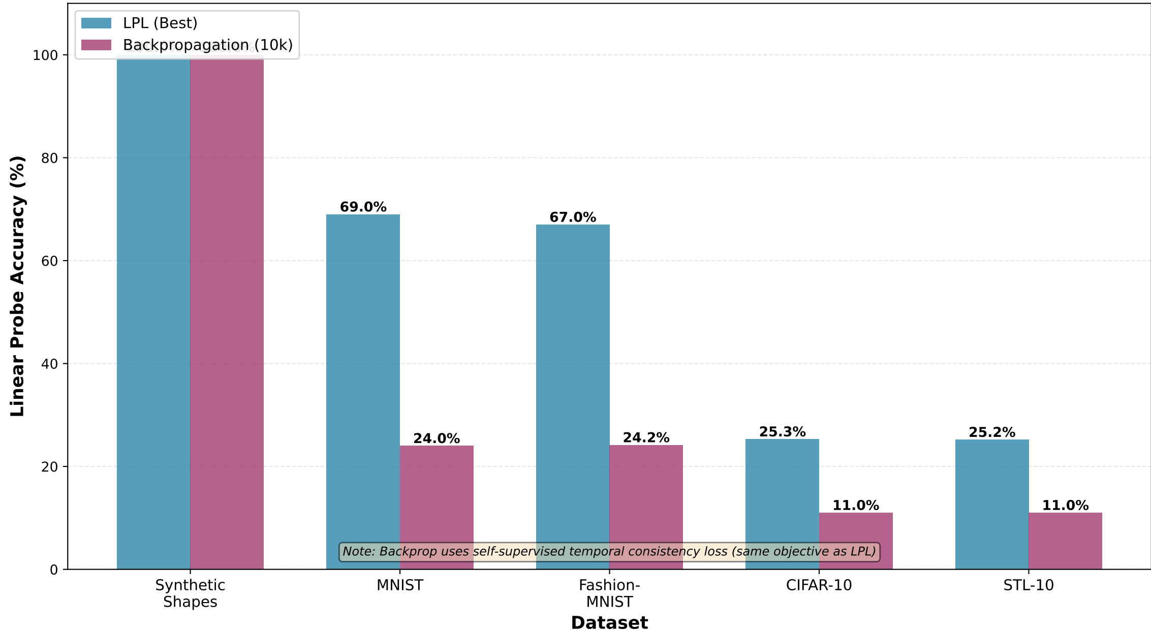
LPL vs Backpropagation: Best Performance Comparison
