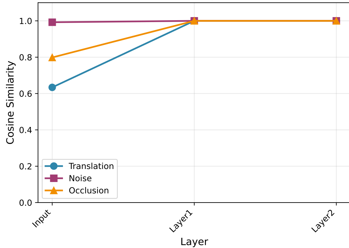
MLP (2-layer)
