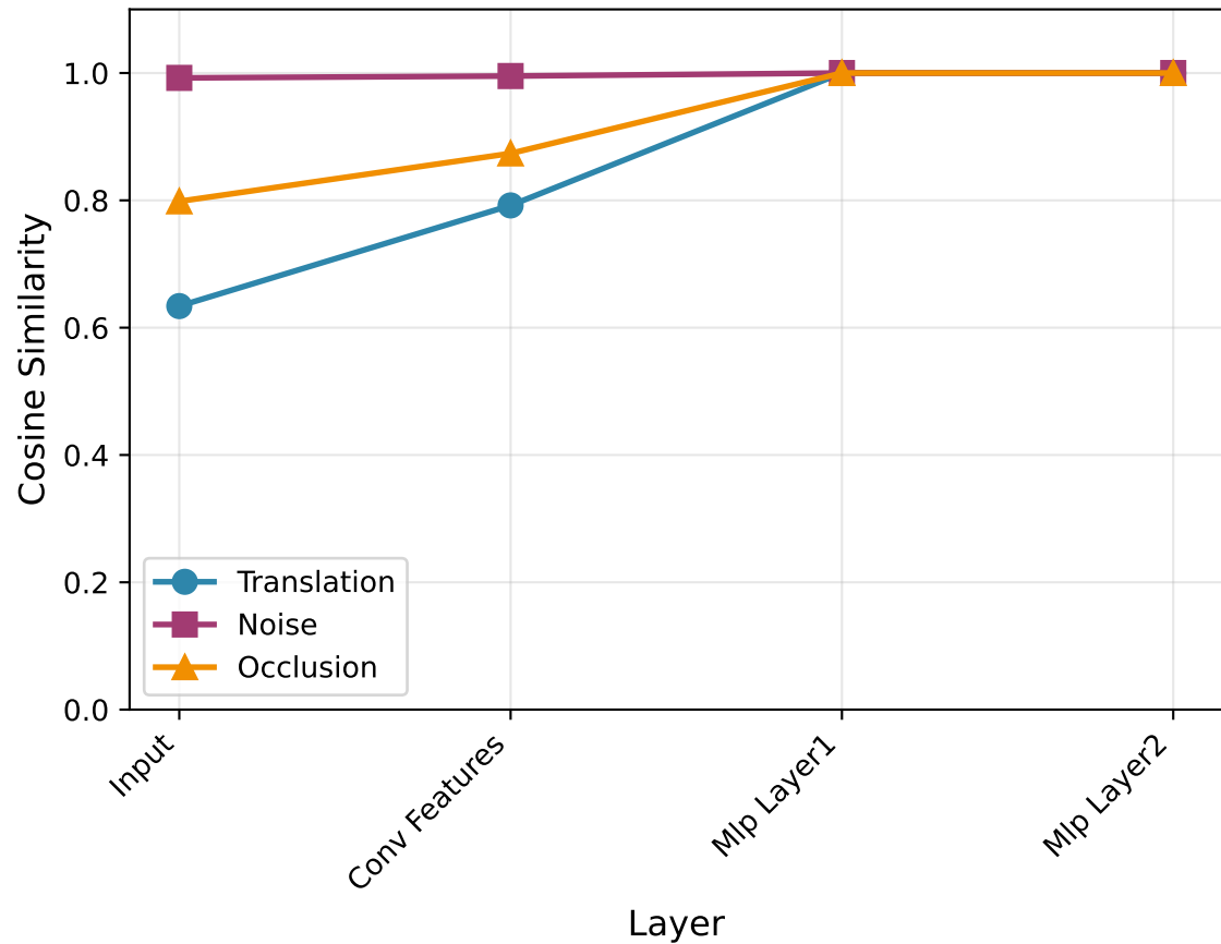
Conv-MLP
