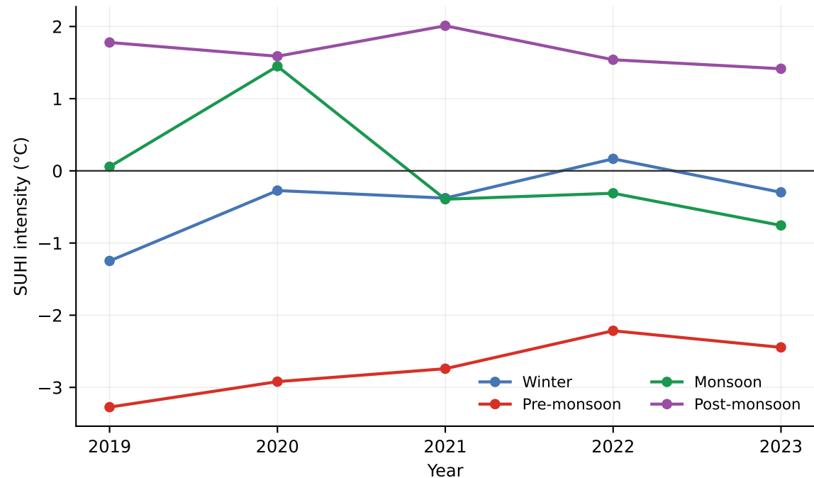
Interannual variation in seasonal SUHI (Terra day)
