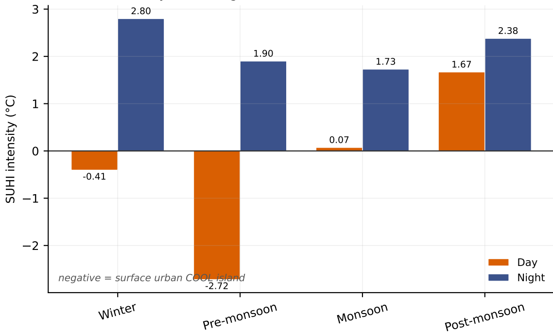
Day versus night SUHI, Terra MODIS (2019–2023)
