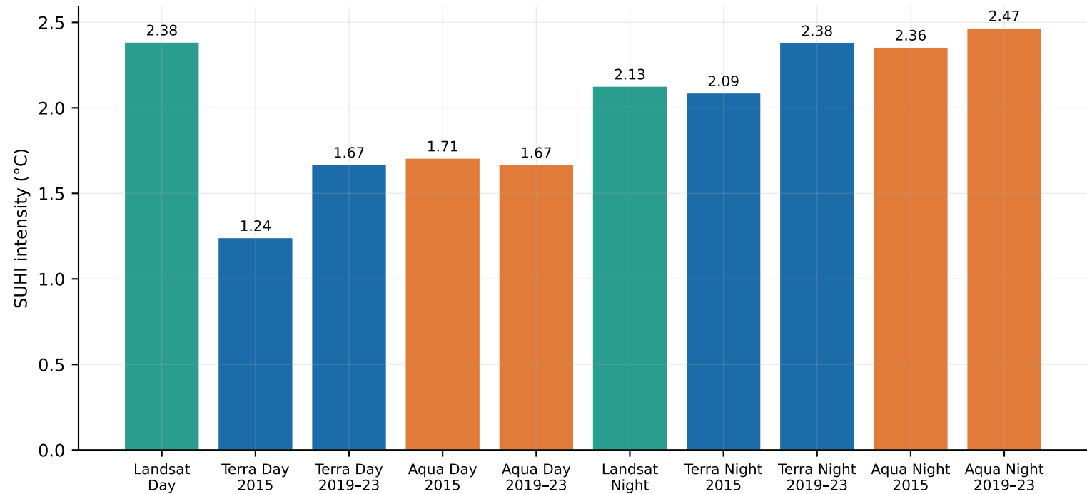
Post-monsoon SUHI: Landsat (8–9 Oct 2015) against matched MODIS rows
