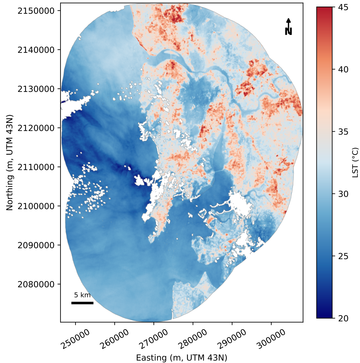
Landsat day LST — 8 October 2015
