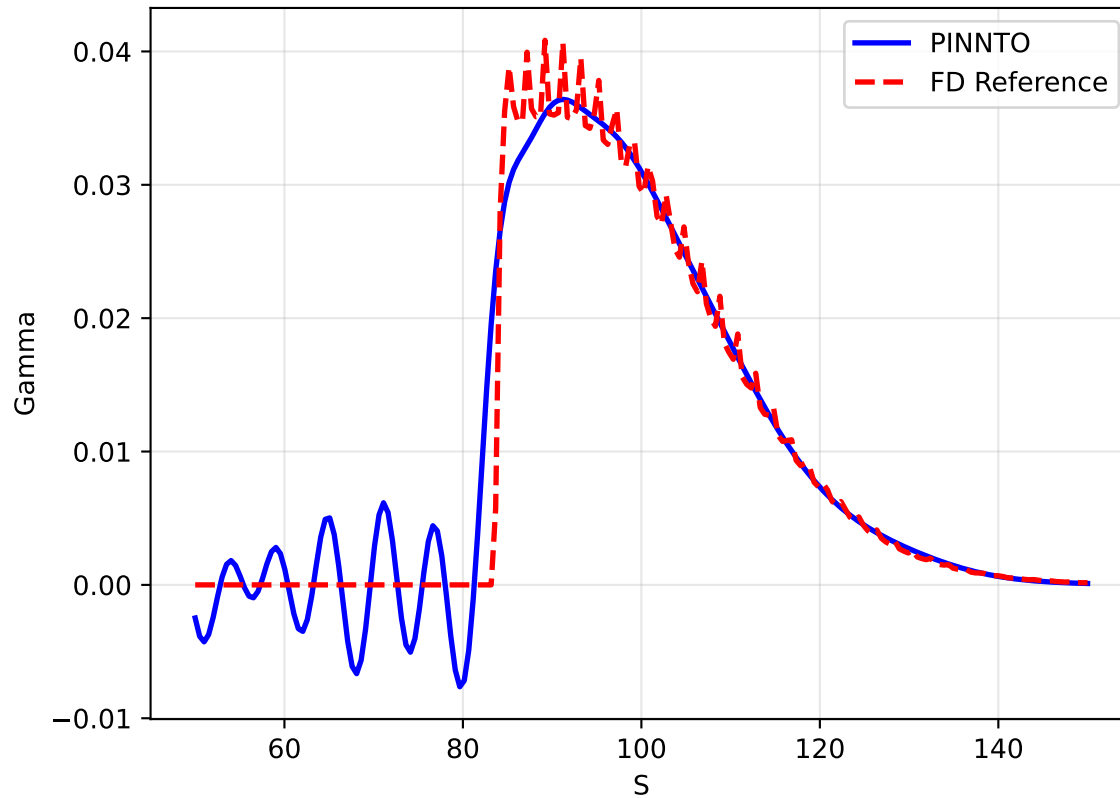
Gamma at \tau=0.5
