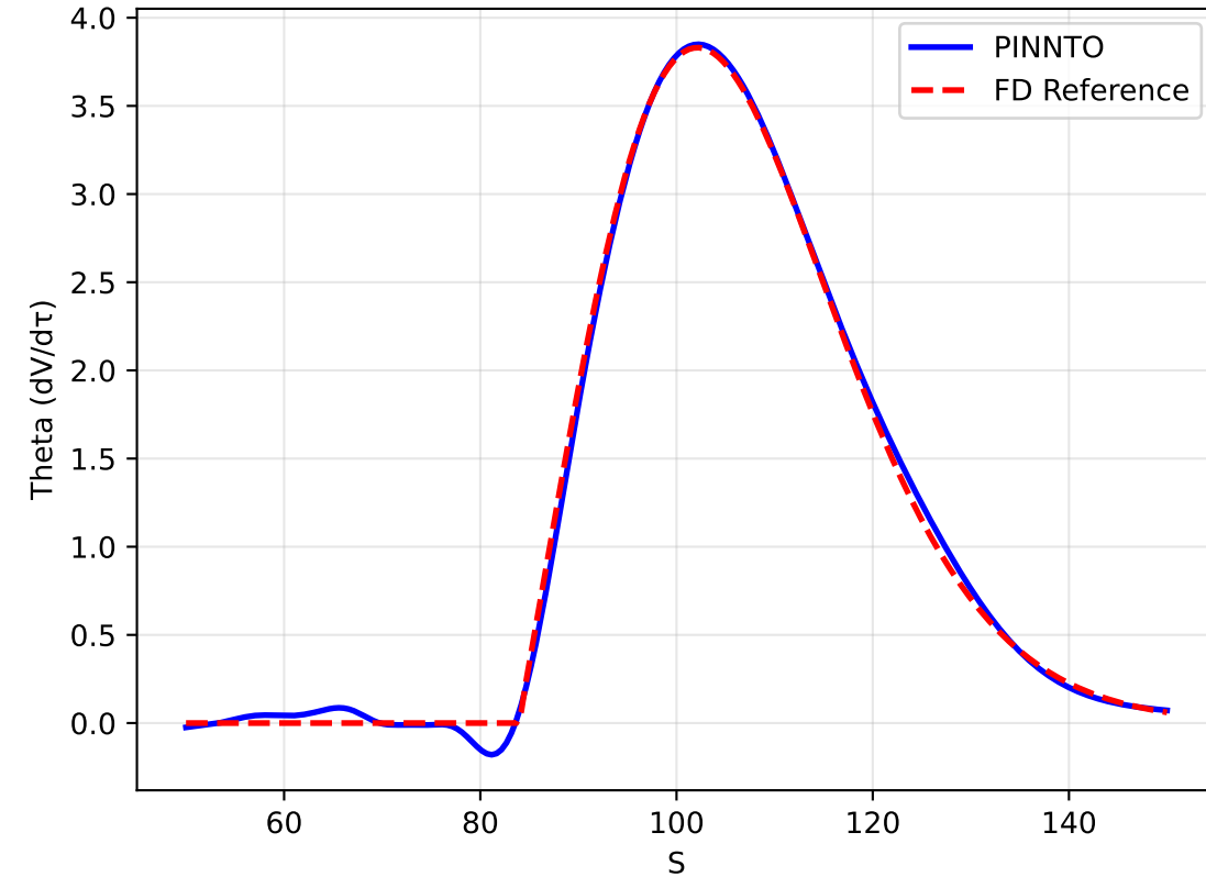
Theta ( dV/d\tau ) at \tau=0.5
