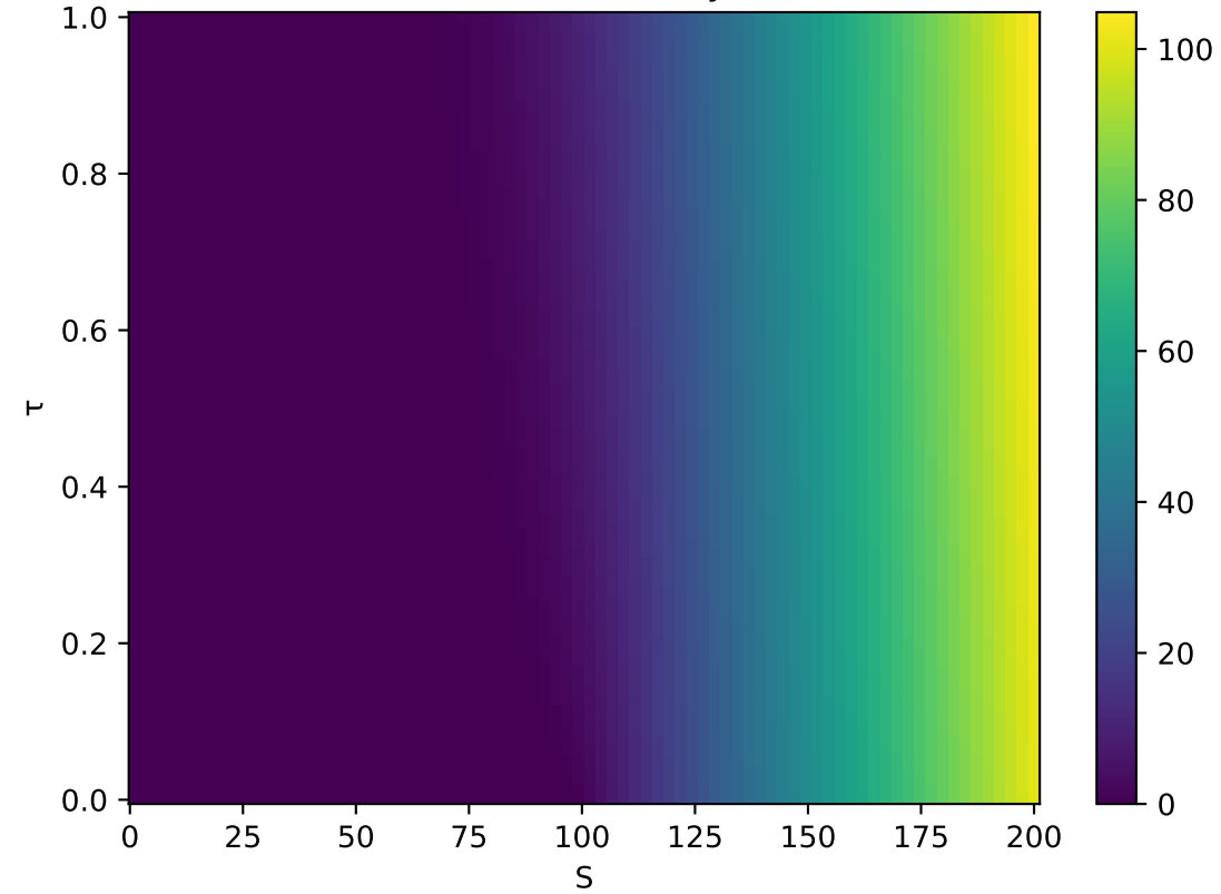
Black-Scholes Analytical
