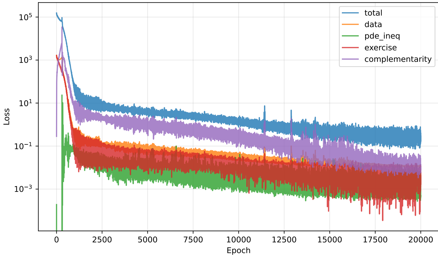
American Put PINN — Loss Convergence (Curriculum Learning)
