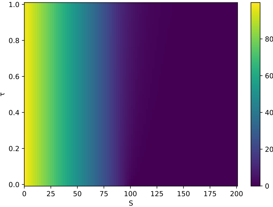
PINNTO American Put
