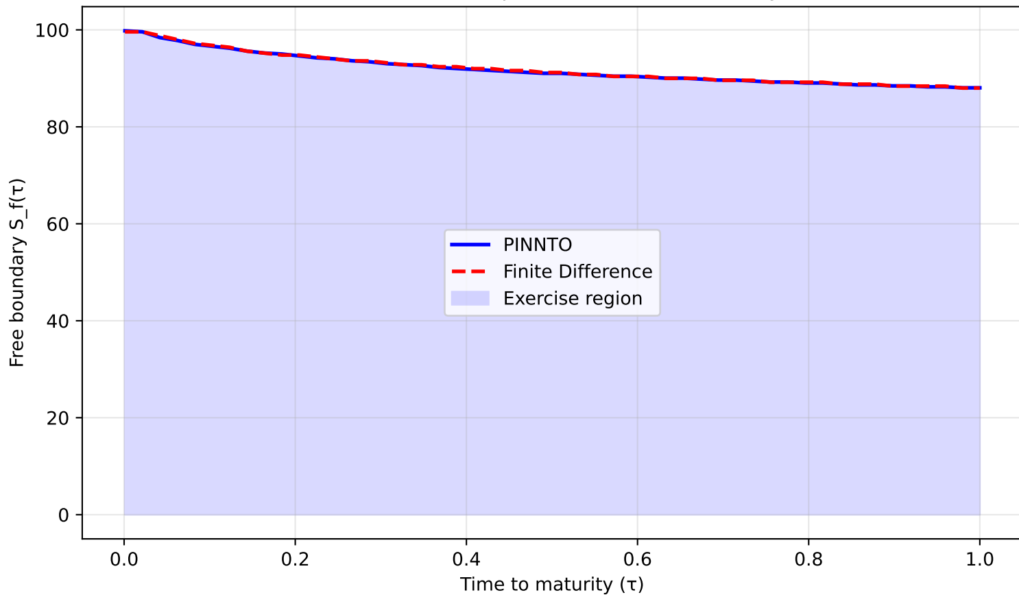
American Put: Optimal Exercise Boundary
