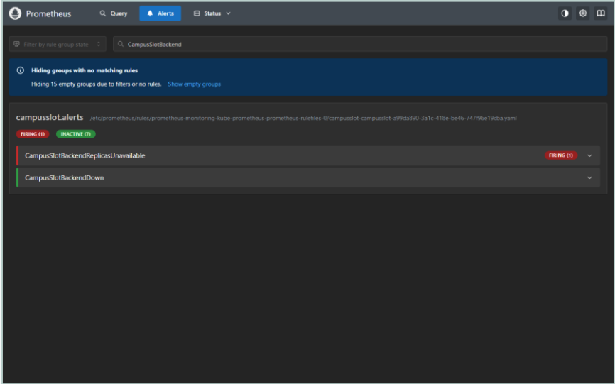
Prometheus: the alert firing during the drill
