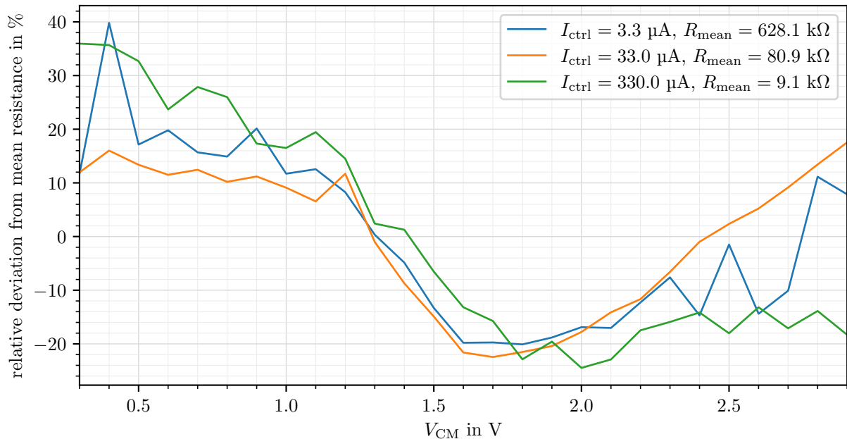
Linearity with respect to V_{\text{CM}} for V_{\text{DM}} = 0.5 V
