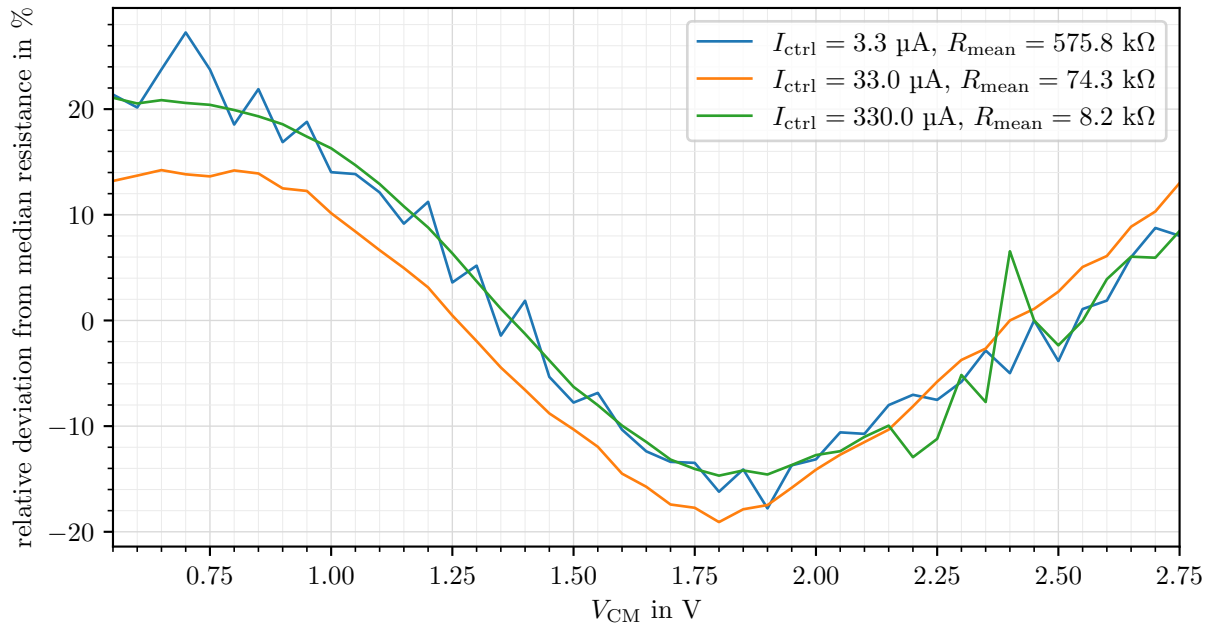
Linearity with respect to V_{\text{CM}} for V_{\text{DM}} = 1.0 V
