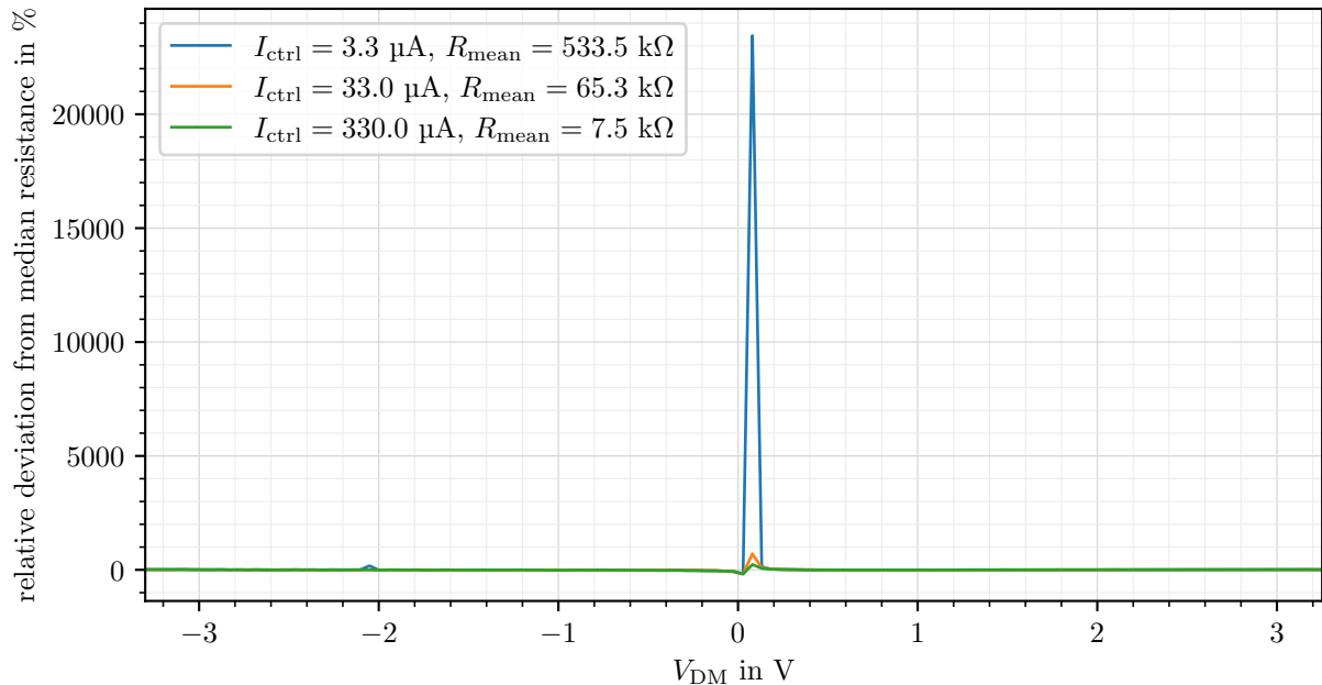
Linearity with respect to V_{\text{DM}} for V_{\text{CM}} = 1.65 \text{ V}
