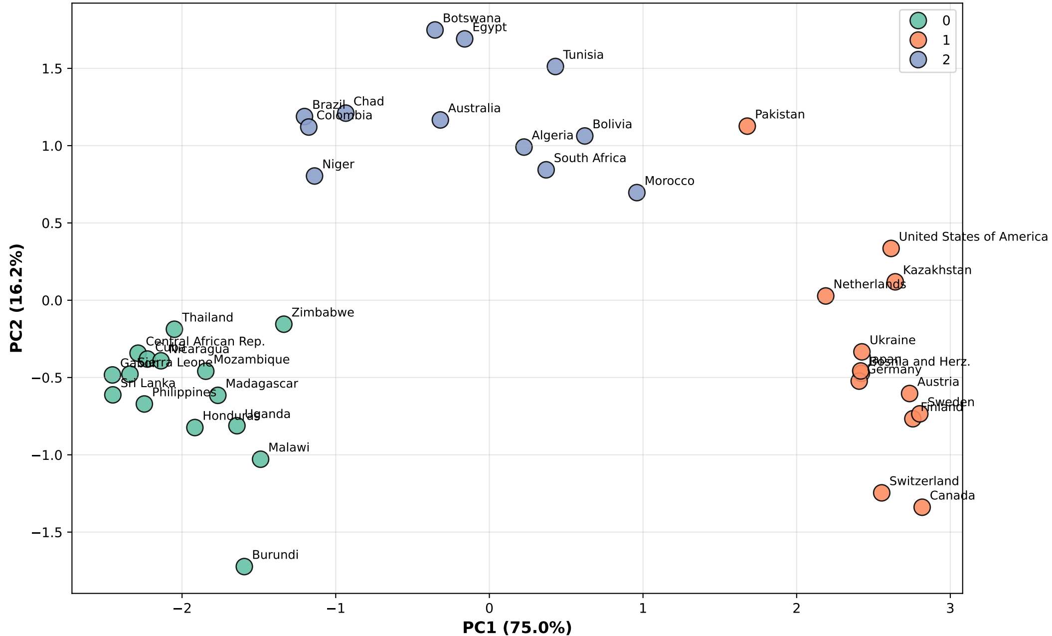
Clustering by health-relevant features (Best k found by model) (Sil=0.564)
