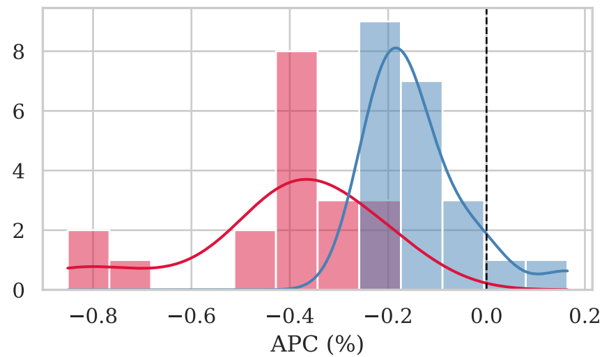
Runoff / Flood
