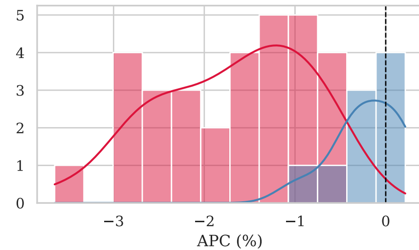
Wind / Pressure
