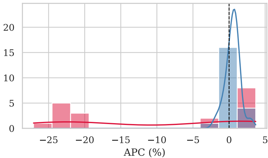
Energy Fluxes
