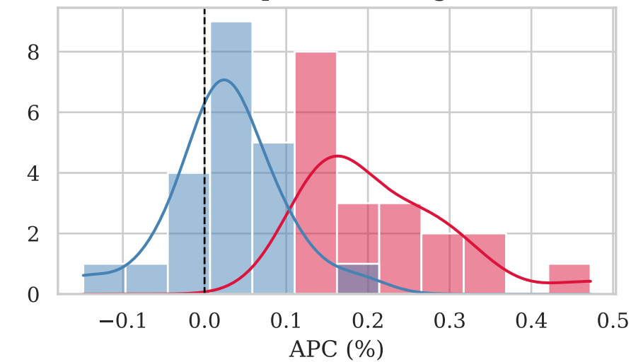
Soil / Moisture
