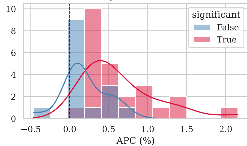
Precipitation / Drought
