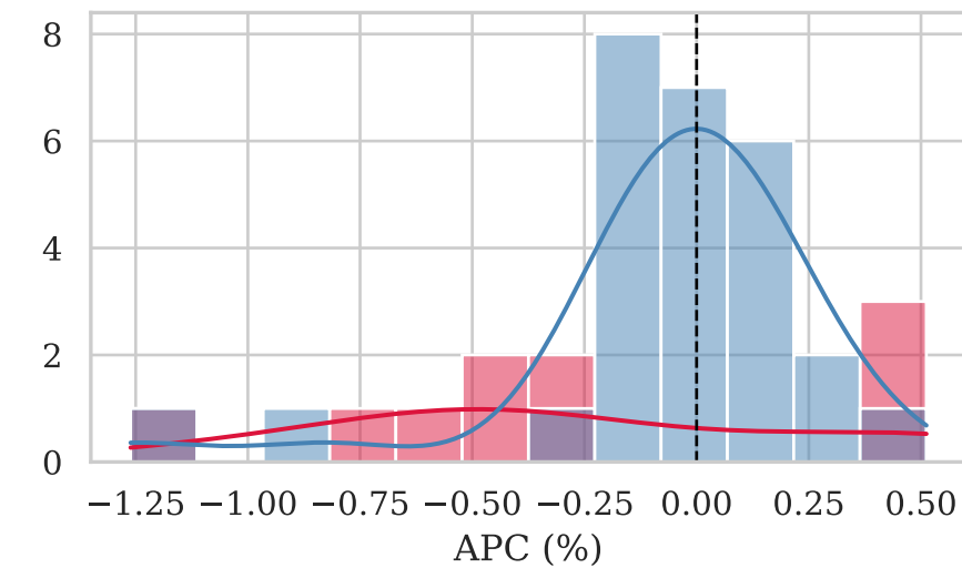
Soil / Moisture
