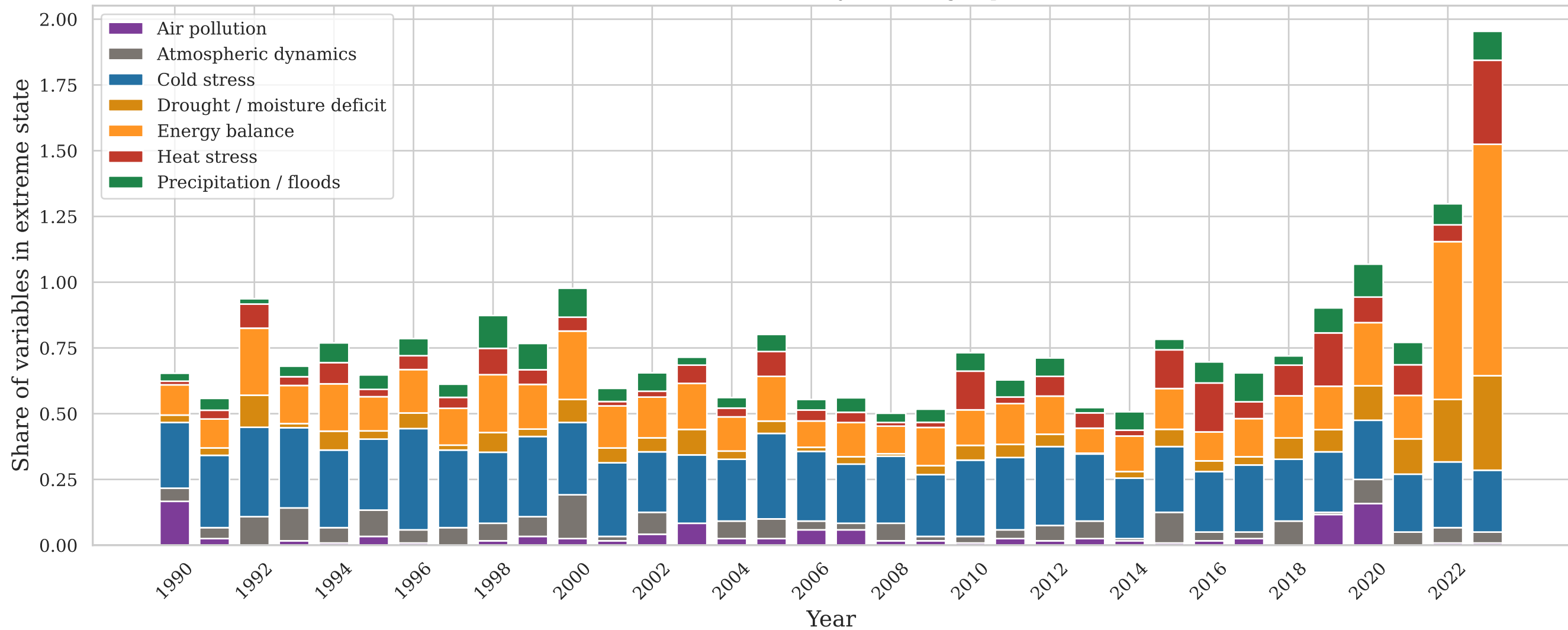
Structure of climate extremes by thematic group (normalized)
