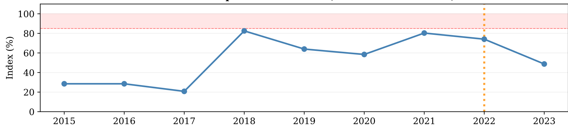
Germany: Composite Heat Stress (Historical Percentiles)
