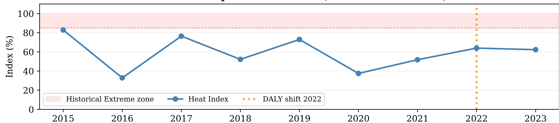
Finland: Composite Heat Stress (Historical Percentiles)
