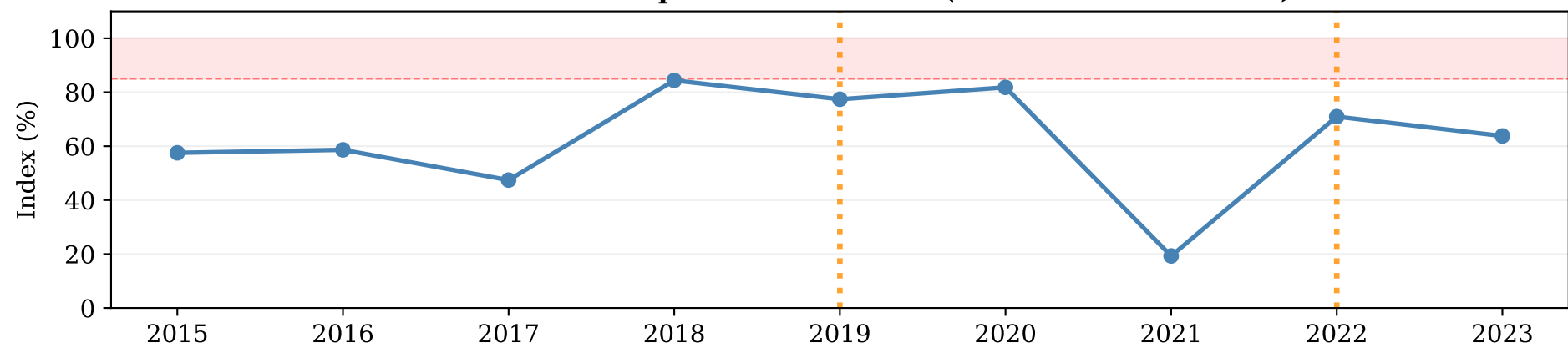
Switzerland: Composite Heat Stress (Historical Percentiles)
