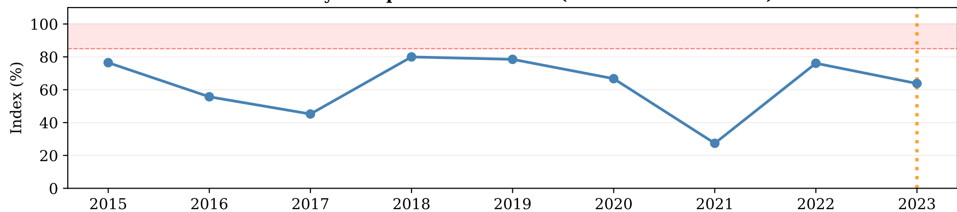
Netherlands: Composite Heat Stress (Historical Percentiles)
