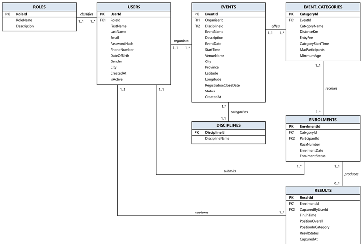
RaceDay - Entity Relationship Diagram
