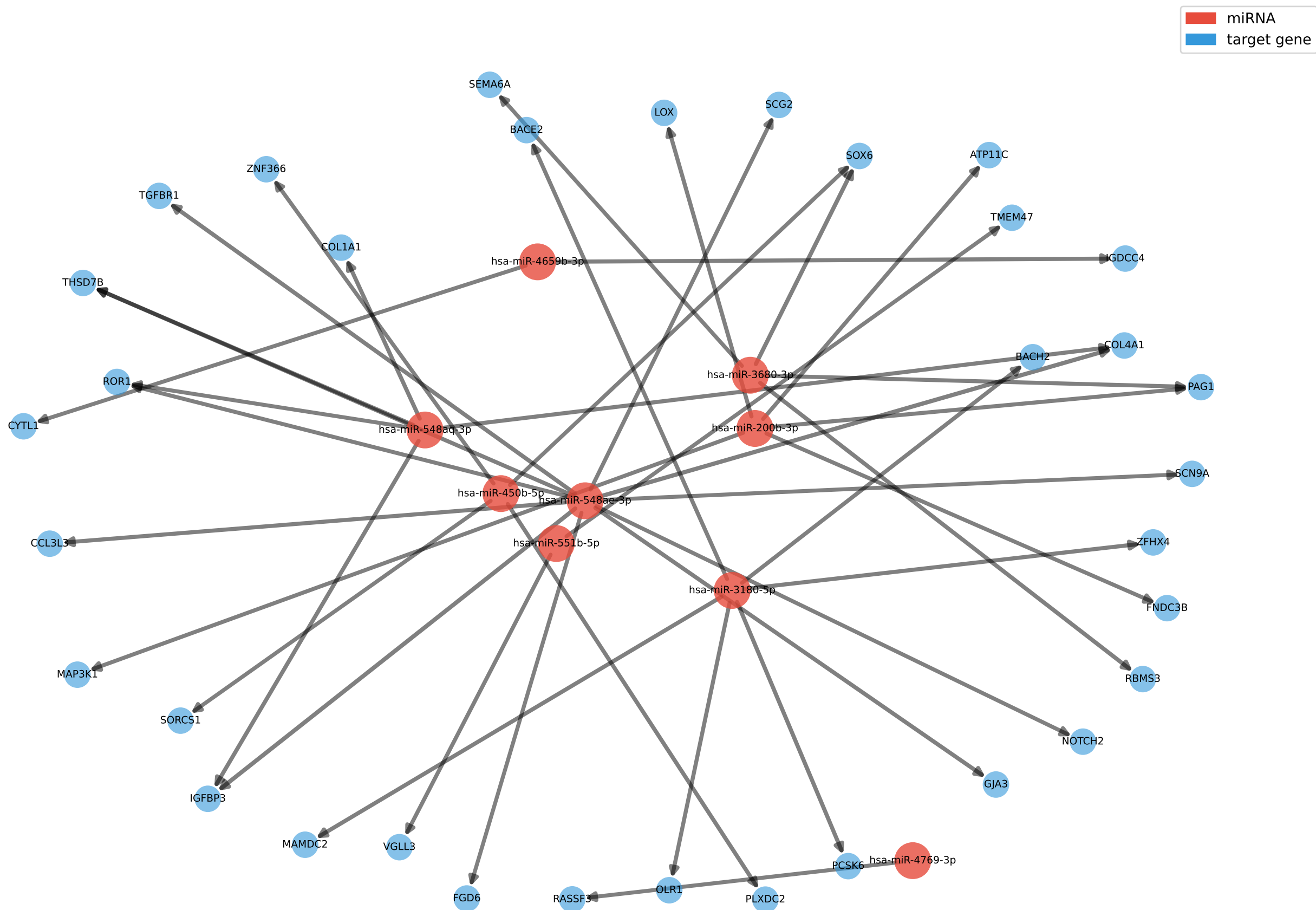
miRNA regulatory circuit — CD8_T (top 40 pairs)
