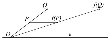
Figure 3.1. Special homology
