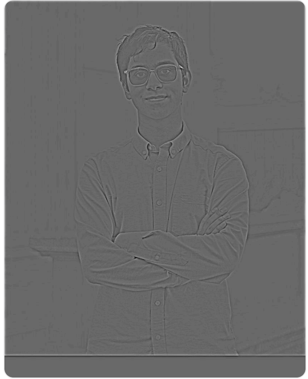
HIGH-PASS (AAYAN)
