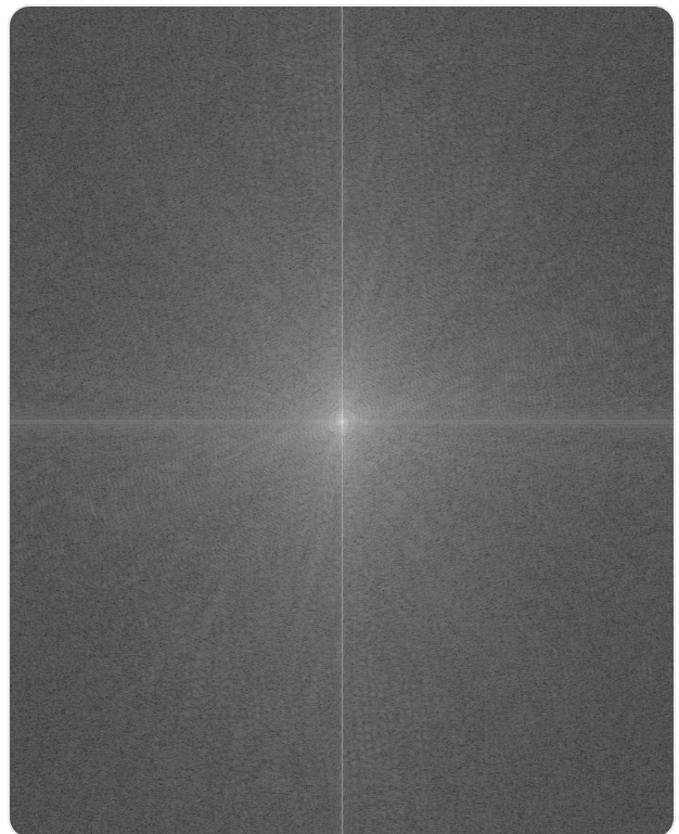
FFT · AAYAN
