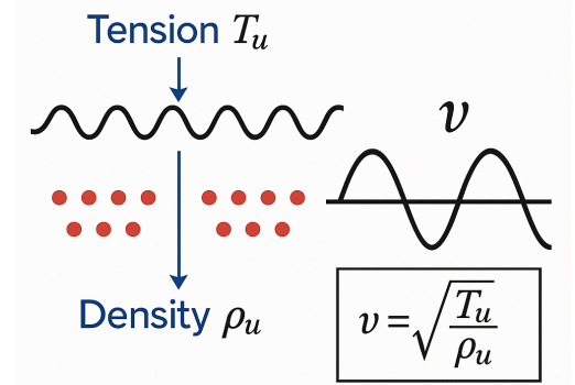
Figure 2: Dimensional derivation of wave speed in the ultronic medium. The relation c = \sqrt{\frac{T_u}{\rho_u}} forms the mechanical foundation from which light speed, gravitational coupling, and Planck’s constant are derived.
