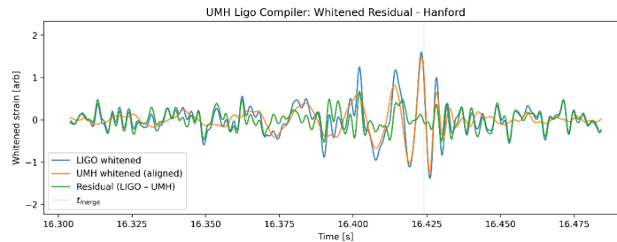
Figure 7: Whited time-domain comparison of LIGO Hanford strain (blue), the aligned UMH chirp (orange), and the residual (green) in a zoomed window around the merger. The same single global source–observer calibration based on Pantheon+ and single global time shift used in the full-window analysis are applied here, with no additional tuning. The residual remains noise-like through the merger, indicating that the UMH waveform captures the local phase evolution and amplitude structure without phenomenological corrections or parameter maximization.
