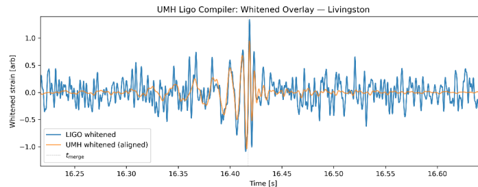
Figure 8: Whited time-domain comparison of LIGO Livingston strain (blue) and the aligned UMH chirp (orange) over the full inspiral–merger window. A single global source–observer calibration based on Pantheon+ (fixing amplitude normalization, frequency evolution, phase accumulation, and time dilation) and a single global time shift are applied across all detectors under the physics-strict alignment rule. The UMH waveform reproduces the observed large-scale chirp morphology, merger timing, and peak amplitude without any stretching, PN tuning, or phenomenological adjustments.
