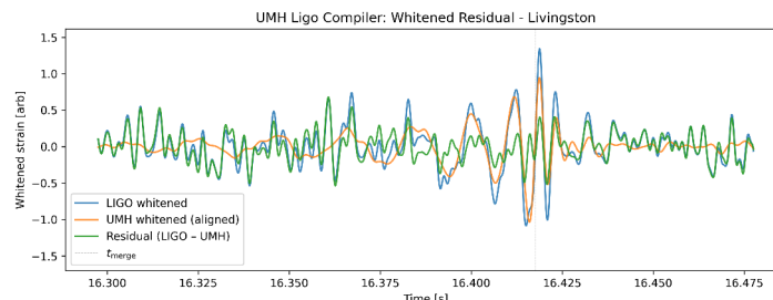
Figure 9: Whited time-domain comparison of LIGO Livingston strain (blue), the aligned UMH chirp (orange), and the residual (green) in a zoomed window around the merger. The same single global source–observer calibration based on Pantheon+ and single global time shift used in the full-window analysis are applied here, with no additional tuning. The residual remains noise-like through the merger, indicating that the UMH waveform captures the local phase evolution and amplitude structure without phenomenological corrections or parameter maximization.
