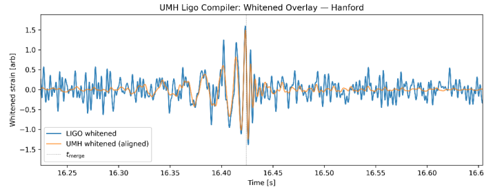
Figure 6: Whited time-domain comparison of LIGO Hanford strain (blue) and the aligned UMH chirp (orange) over the full inspiral–merger window. A single global source–observer calibration based on Pantheon+ (fixing amplitude normalization, frequency evolution, phase accumulation, and time dilation) and a single global time shift are applied across all detectors under the physics-strict alignment rule. The UMH waveform reproduces the observed large-scale chirp morphology, merger timing, and peak amplitude without any stretching, PN tuning, or phenomenological adjustments.
