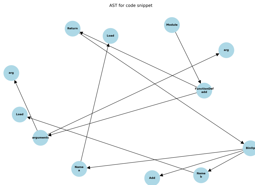
Figure 1: AST example for a simple function
