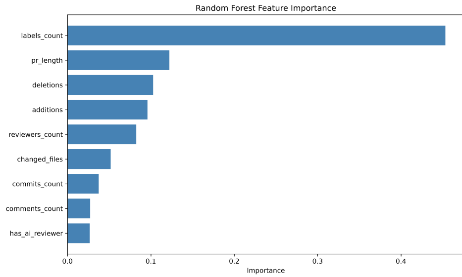
Figure 3: Random Forest feature importance
