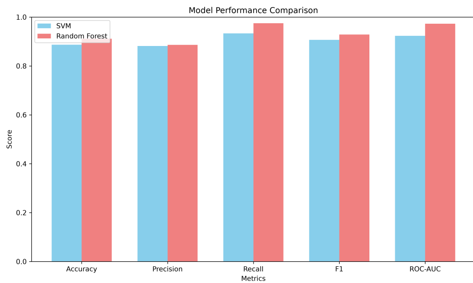
Figure 4: SVM vs Random Forest performance comparison
