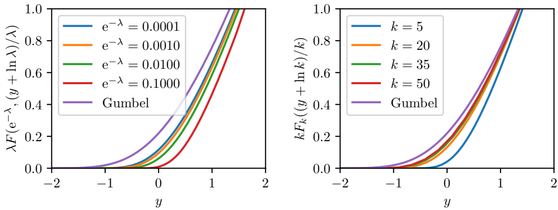
Figure 12.1: The integrated cumulative distribution functions of the continuum limit of the longest run statistics (left) and the longest segment of the broken stick (right) tend to that of the Gumbel distribution.
