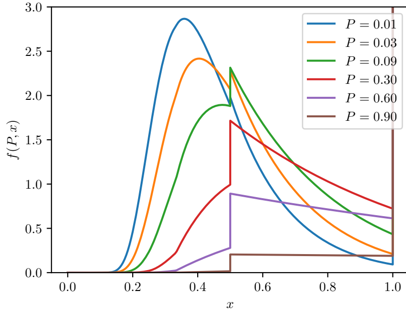
Figure 7.2: Plot of f(P, x) for various values of P .
