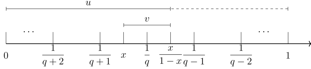
Figure 7.1: Illustration of the interval of integration over u and v when 1/(q+1) < x < 1/q .
