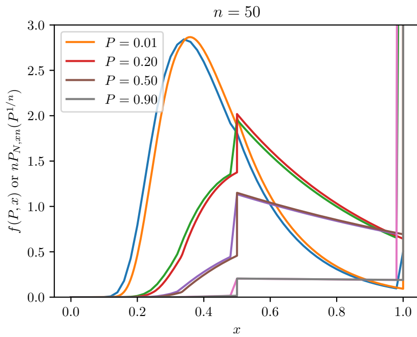
Figure 7.3: Comparing f(P, x) and P_{n,xn}(p) in the same plot for n = 50 . The lines for P_{n,xn}(p) are not legended.
