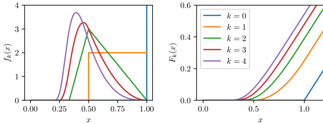
Figure 10.1: Plot of f_k(x) and F_k(x) for various values of k . The legend is shared.
