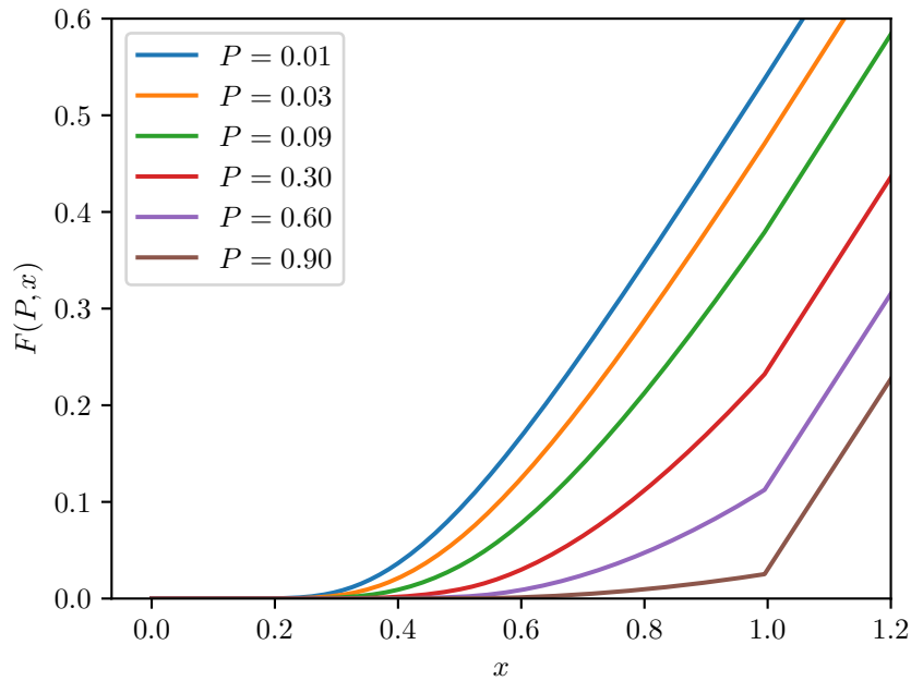
Figure 9.2: Plot of F(P, x) for various values of P .
