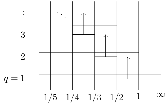
Figure 6.1: Illustration of solving the function g piece by piece using the ADM. The three horizontal lines from bottom to top for each q represent, respectively, the range of x , the largest interval of integration over u , and the largest interval of integration over v , as they appear in Equation 4.7 when g^{(q)} is being solved.
