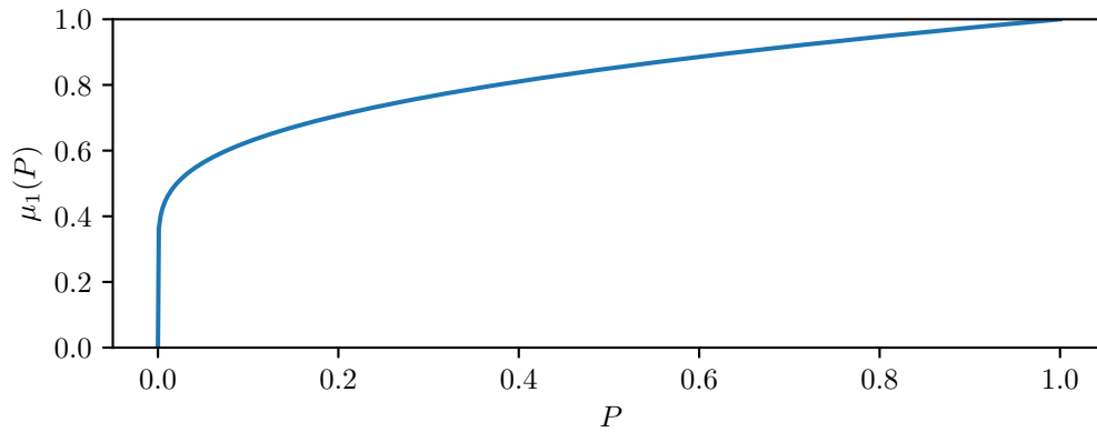
Figure 9.1: The dependence on P of the mean \mu_1(P) of the distribution with probability density f(P, x) .
