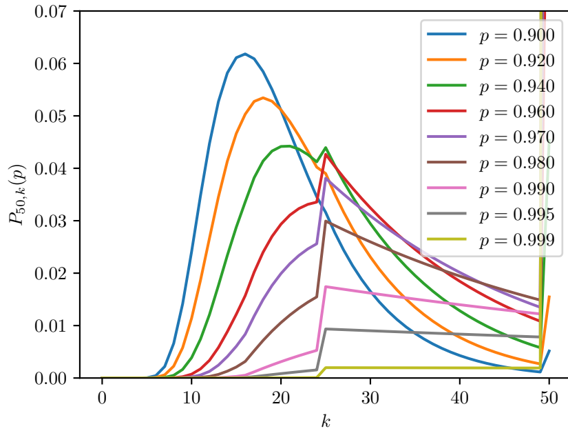
Figure 3.2: The probability distribution P_{n,k}(p) when n = 50 .
