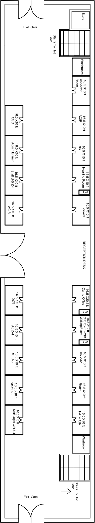
RTO-II Nipa Building Floor Plan Ground Floor
