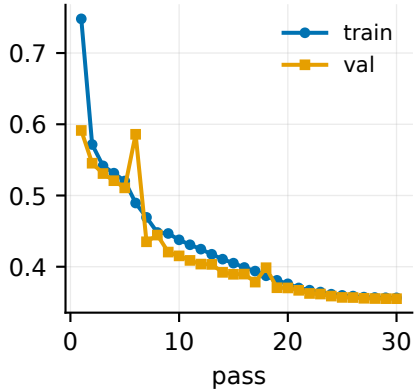
Loss
