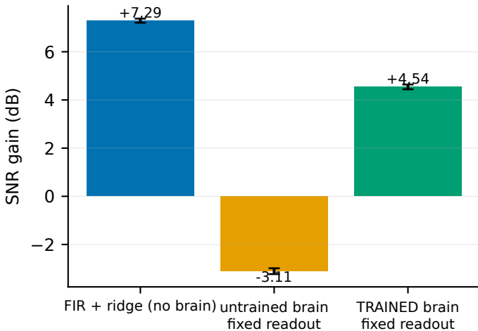
BOTH: test SNR gain (n=500 epochs)
