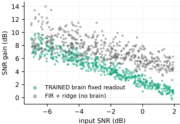
BOTH: per-epoch gain
