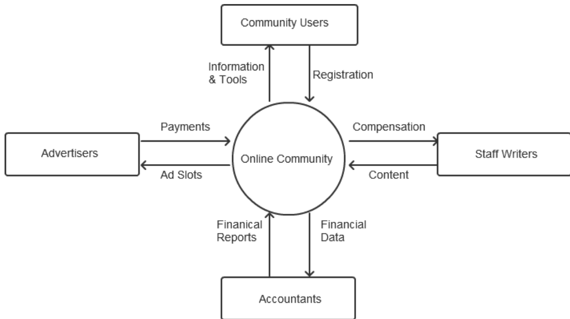
Figure 4.3: DFD Level 0
