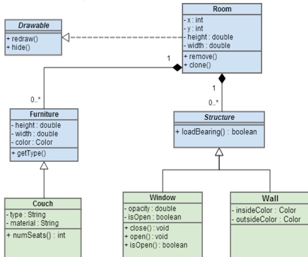
Figure 4.8: Interface Design Diagram
