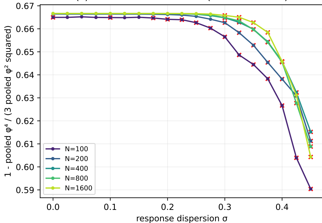
(c) Pooled Binder statistic (denominator 3)
