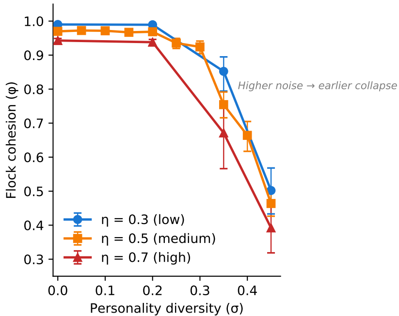
B Noise \times diversity interaction
