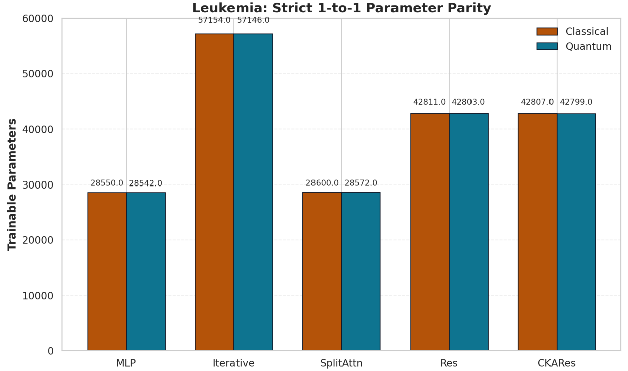
Figure 4 — 1-to-1 Parameter Ablation. Both classical and quantum architectures utilize an effectively identical number of trainable parameters, isolating the quantum bottleneck as the sole driver of performance variance.
