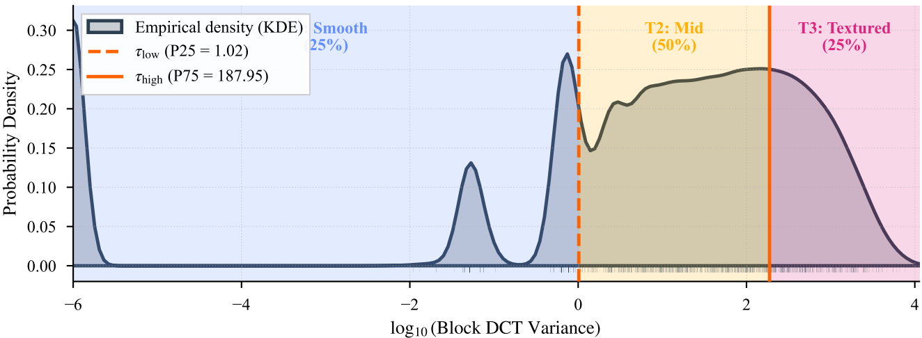
Distribution of 8\times 8 Block DCT Variance in AI-Generated Images (Stable Diffusion v2.1, n = 50 images, N = 204,800 blocks)
