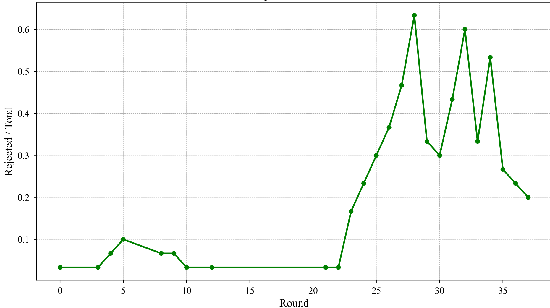
Defense Rejection Ratio vs Round
