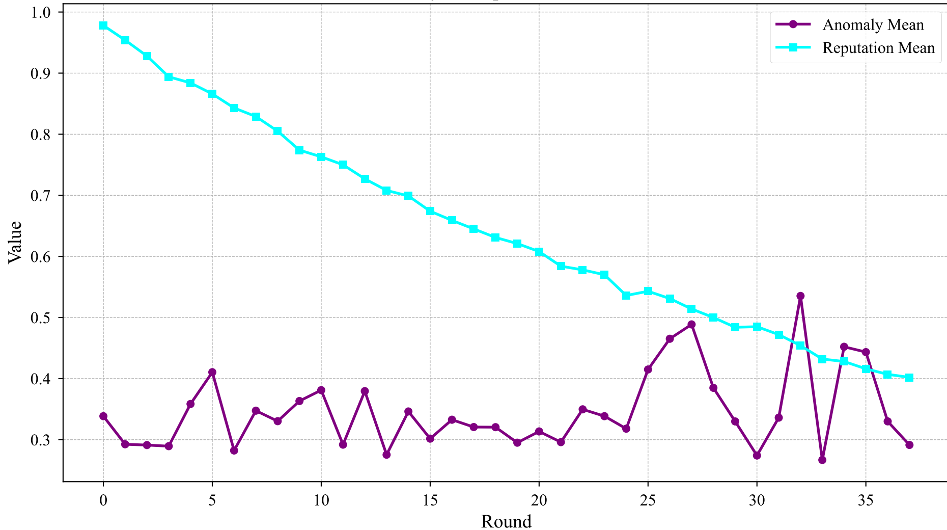
Anomaly & Reputation vs Round
