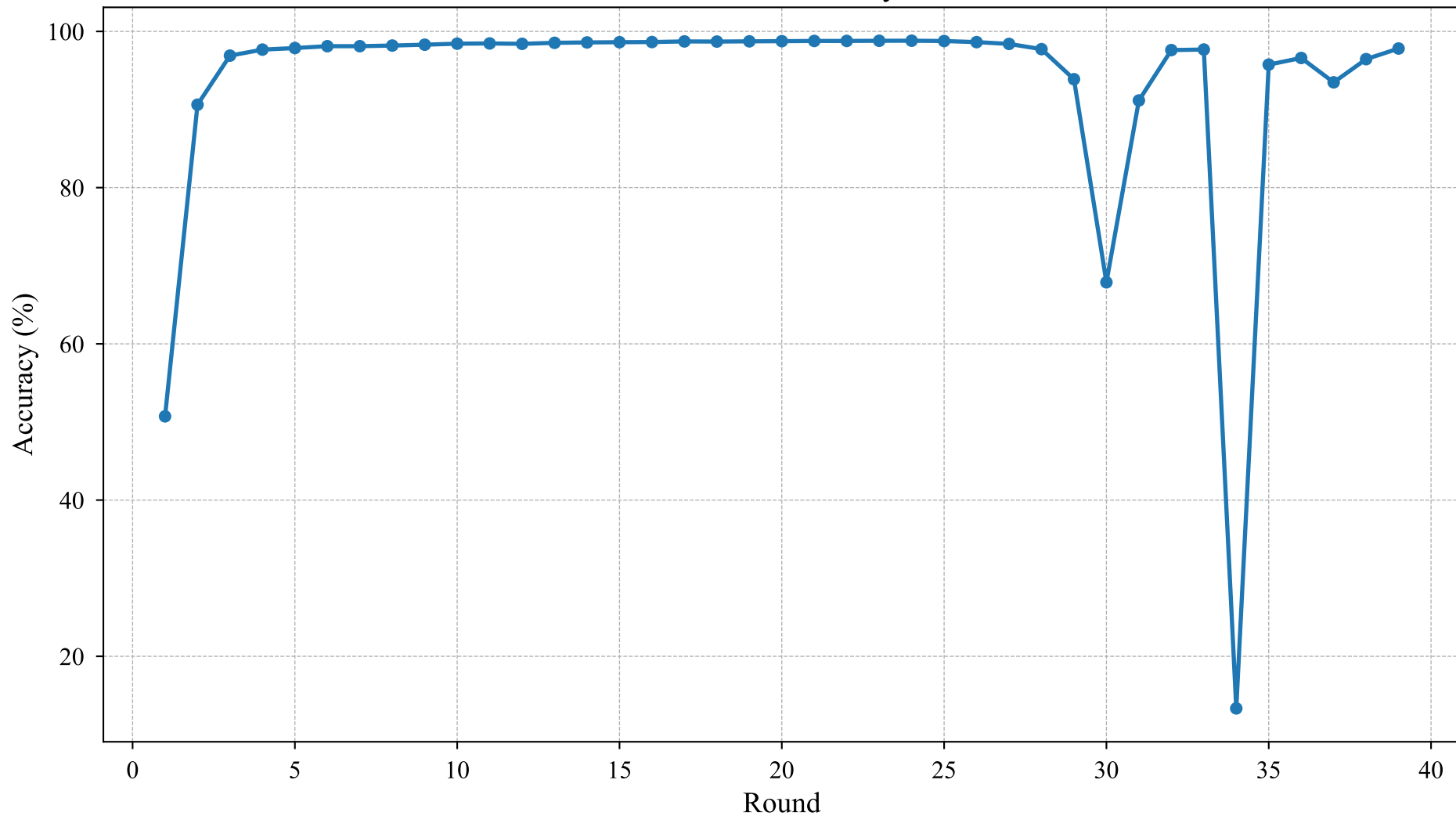
Global Validation Accuracy vs Round
