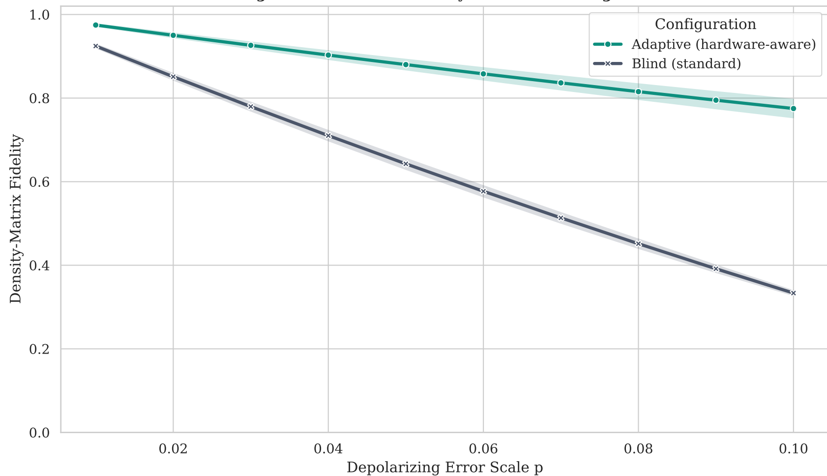
Figure 1: Bell-State Fidelity Across Noise Regimes
