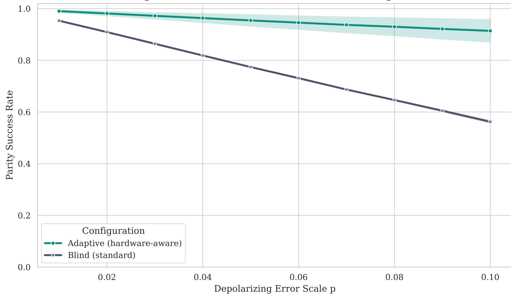
Figure 2: Bell-State Success Rate Across Noise Regimes
