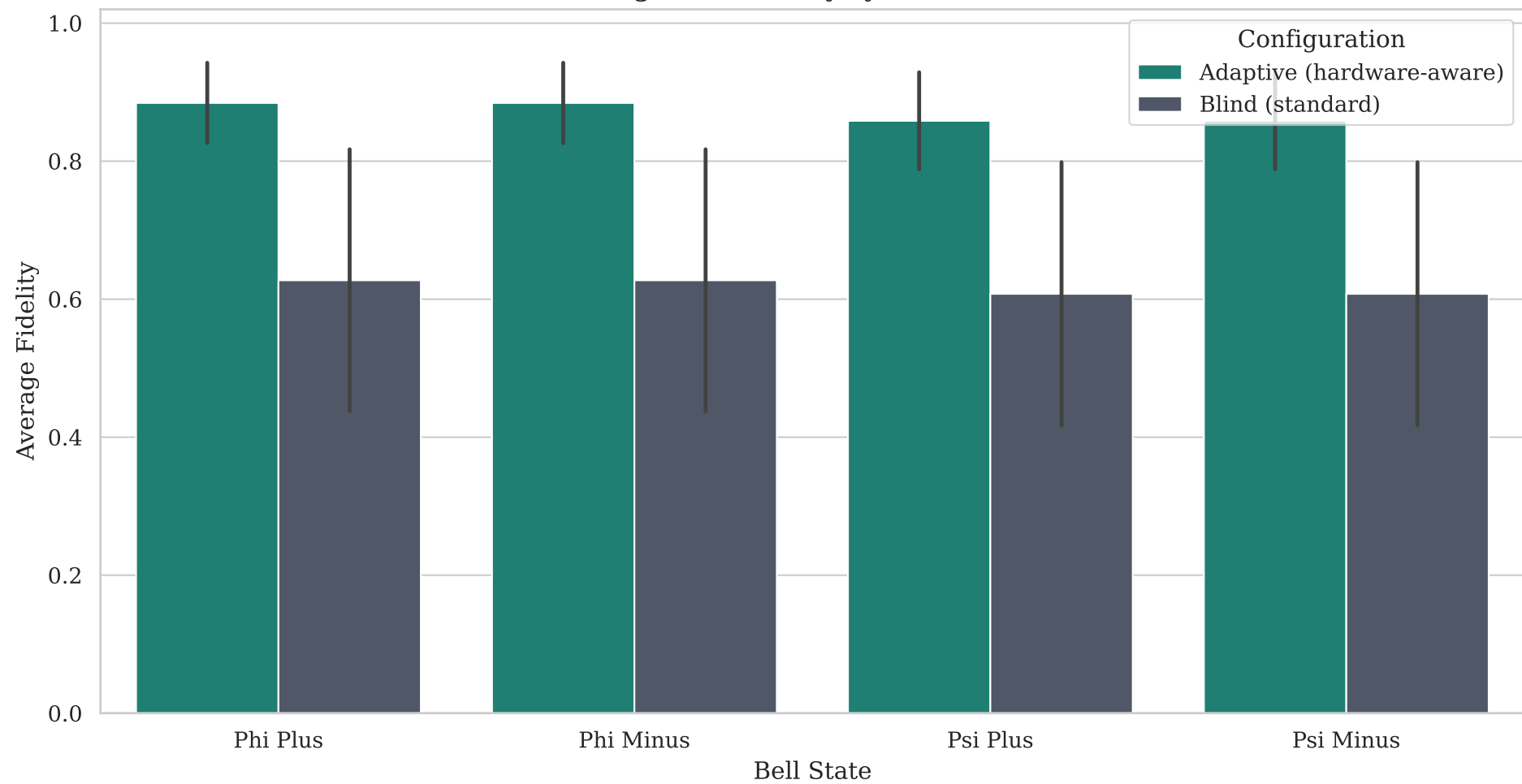
Figure 4: Fidelity by Bell State
