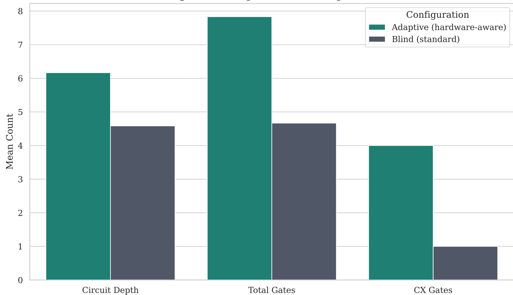
Figure 6: Transpilation Cost Comparison
