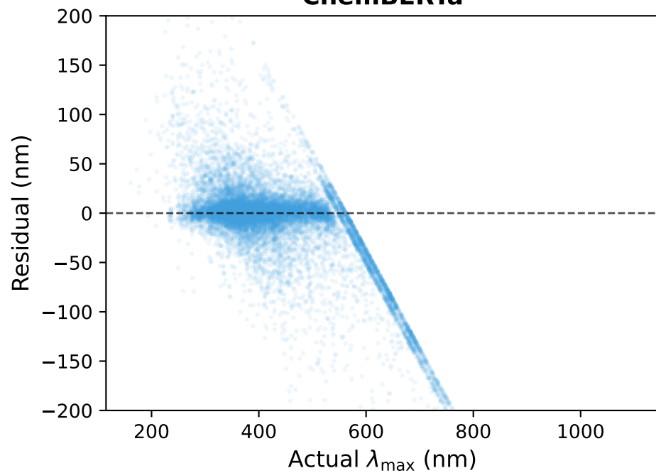
ChemBERTa
