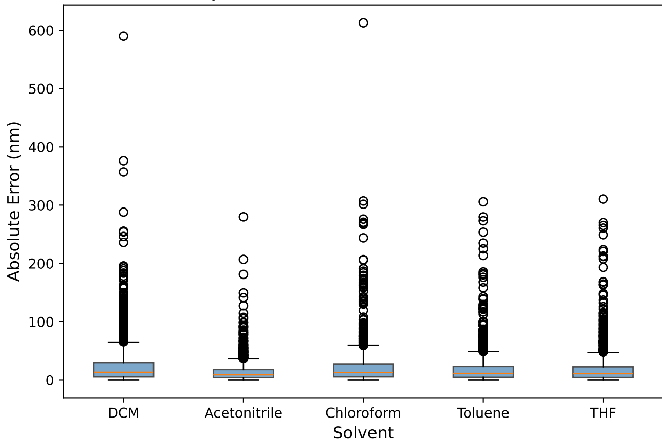
Error by Solvent — BiGRU + Solvent (5-Fold CV)
