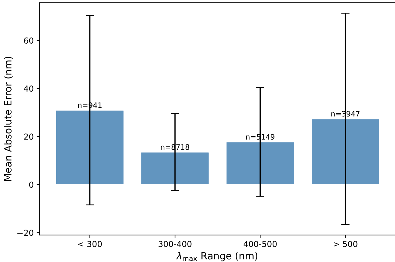
Error by Wavelength Range — BiGRU + Solvent (5-Fold CV)
