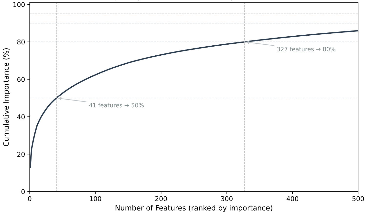
RF Model Sparsity: Few Substructures Explain Most Predictions
