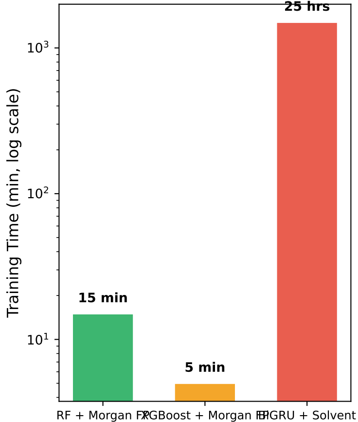
Computational Cost (5-fold CV)
