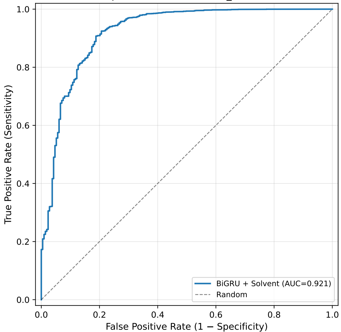
ROC: Photosafety Classification (POS: \lambda_{\text{max}} \in [290, 700] nm)
