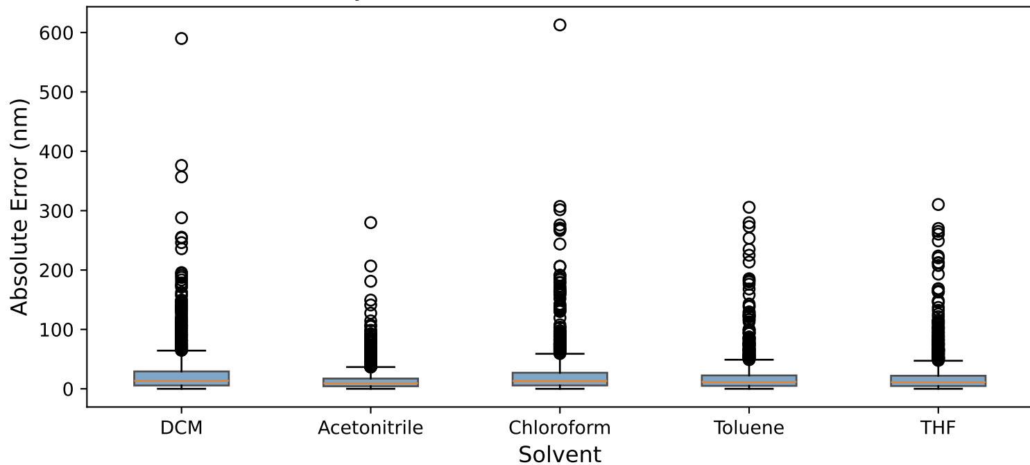
Error by Solvent — BiGRU + Solvent (5-Fold CV)
