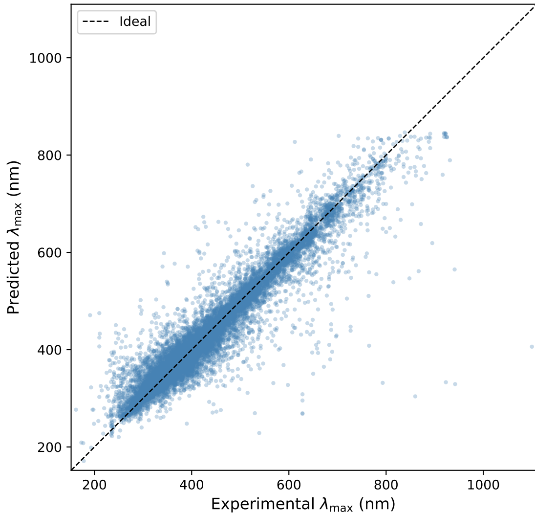
BiGRU + Solvent — 5-Fold CV (RMSE = 33.5 nm)
