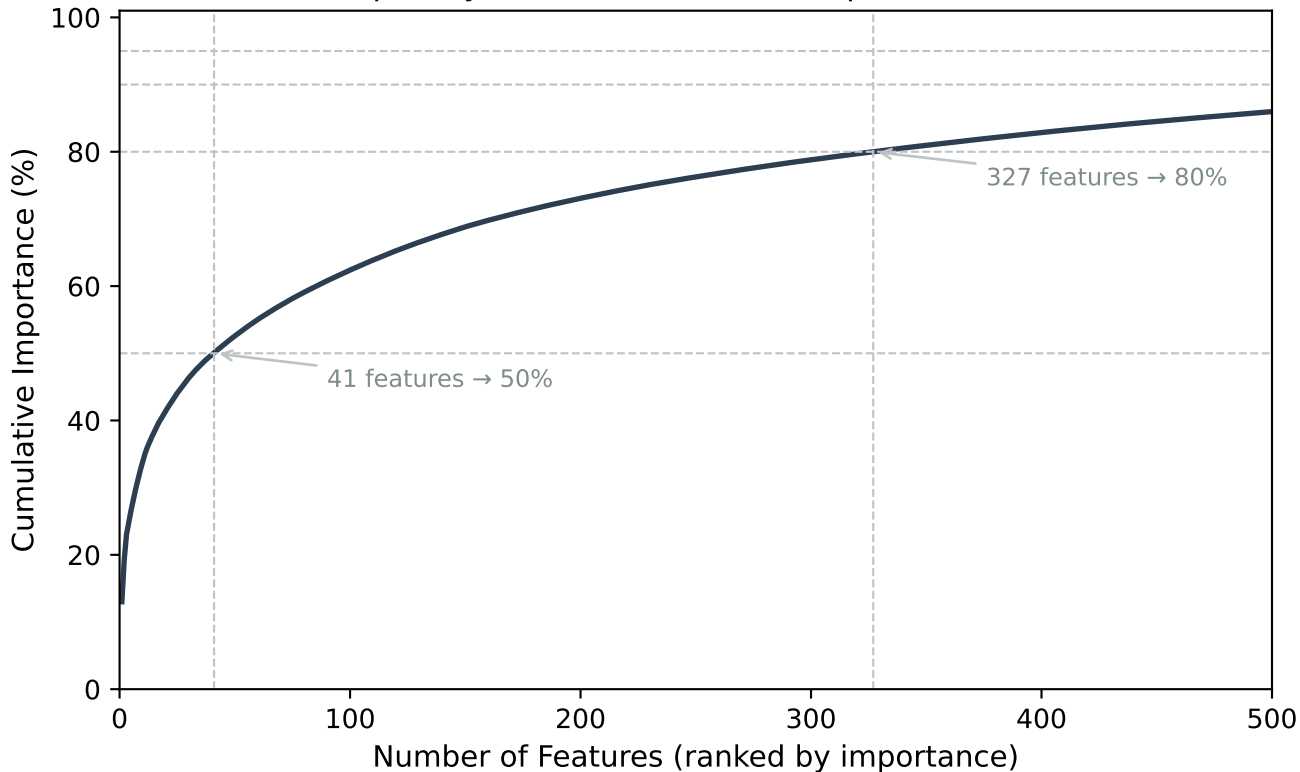
RF Model Sparsity: Few Substructures Explain Most Predictions
